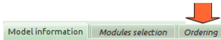
Figure 29: “Ordering” tab
