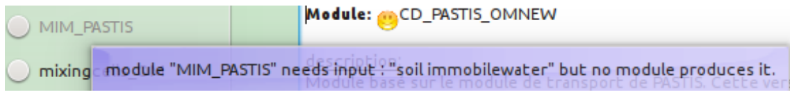
Figure 44: Non-selectable module
