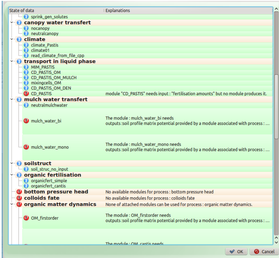
Figure 10: Status report
